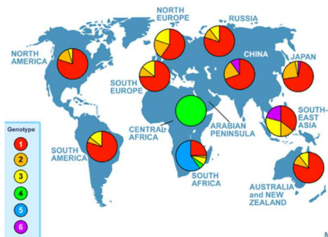
Fig. 1 Global distribution of HCV genotypes. Source: WHO Hepatitis C Fact Sheet no. 164 (July 2012): http://www.who.int/mediacentre/factsheets/fs164/en/index.html . Source image: http://www.gregoryledet.com/?p=60 .
