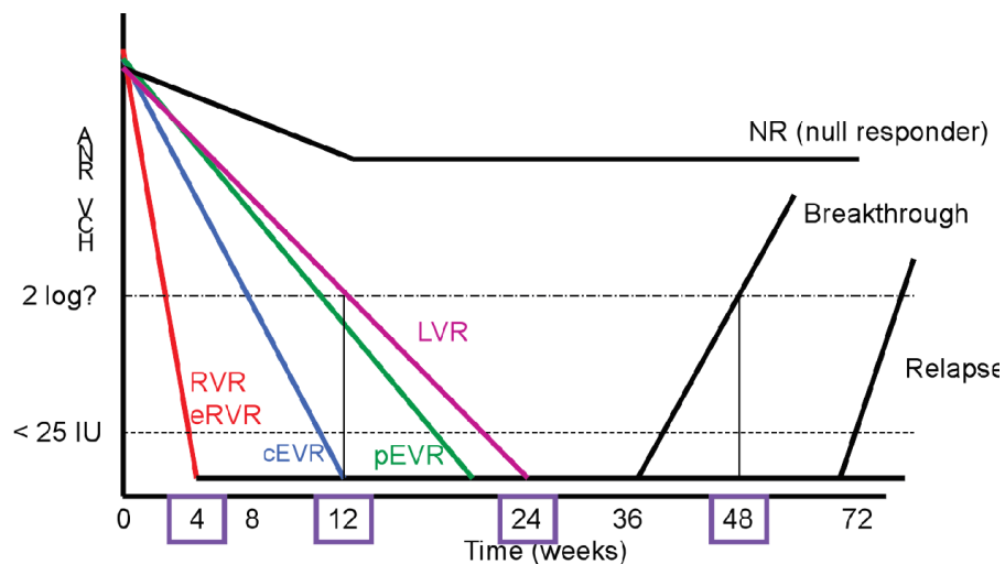
Fig. 3 Pattern of viral responses with peginterferon/ribavirin (PEG-IFN/RBV) therapy.
